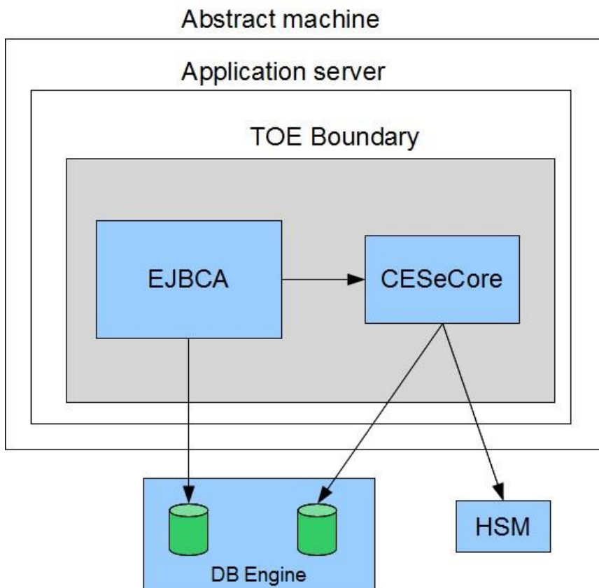
Figure 1, TOE boundary
